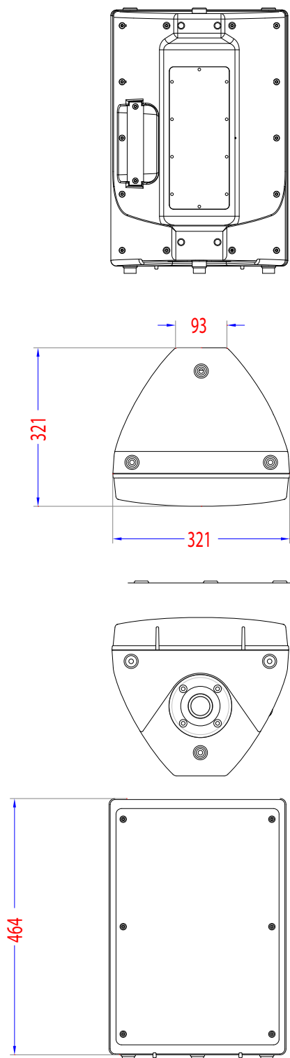
Dimensions (mm)
